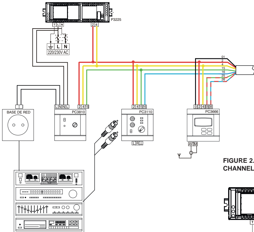
FIGURE 1. CENTRALISED INSTALLATION WITH TWO STEREO CHANNELS (ONE EXTERNAL CHANNEL + PCD3666 TUNER) WITH PC3819 REMOTE CONTROL MODULE.
