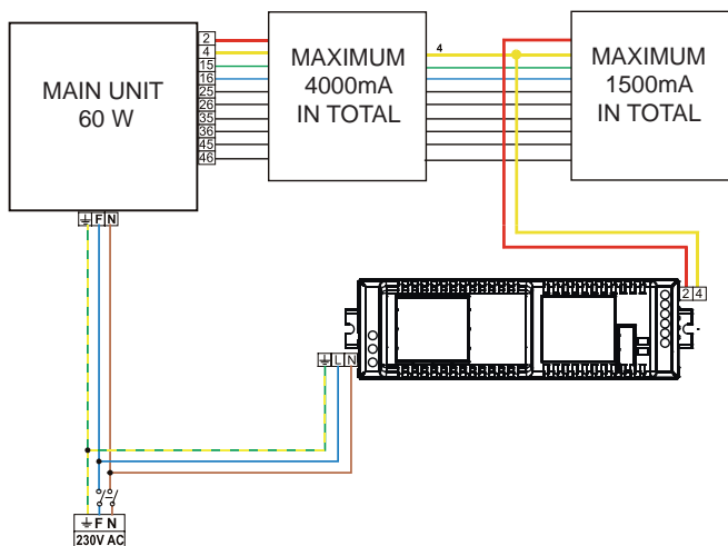
FIGURE 3. INSTALLATION AS AUXILIARY POWER SUPPLY
