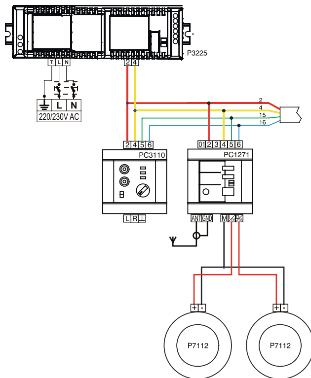
FIGURE 2. CENTRALISED INSTALLATION WITH 1 STEREO CHANNEL CONTROL/PCP1271 LOCAL TUNER CONNECTION.
