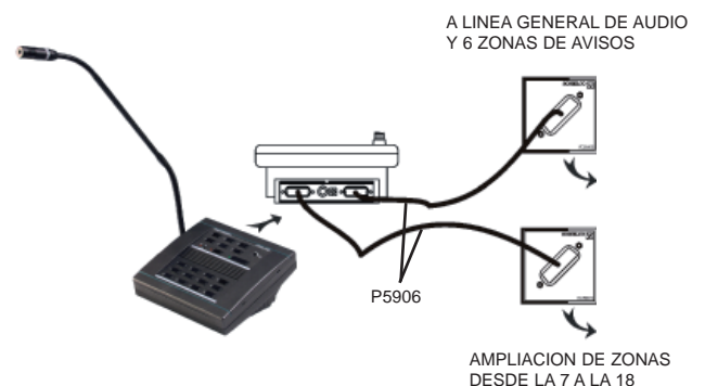
Installation detail with desktop microphone P5580
