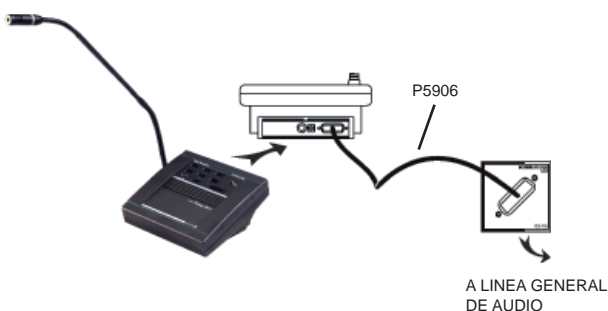
Installation detail with desktop microphones P5552 and P5556
